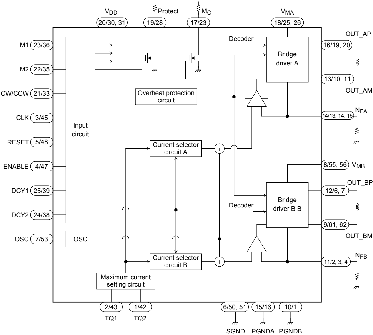
TB6560HQ/TB6560FG
